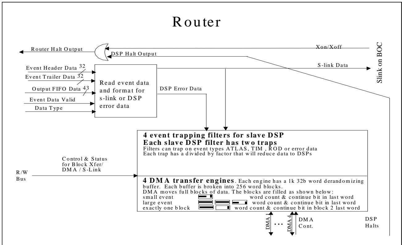
Figure 8: Router
