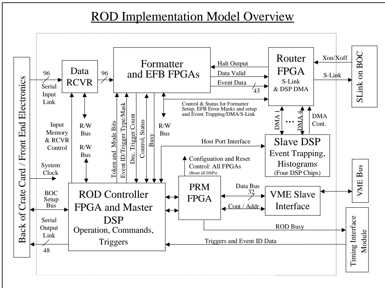
Figure 1: ROD Implementation model
