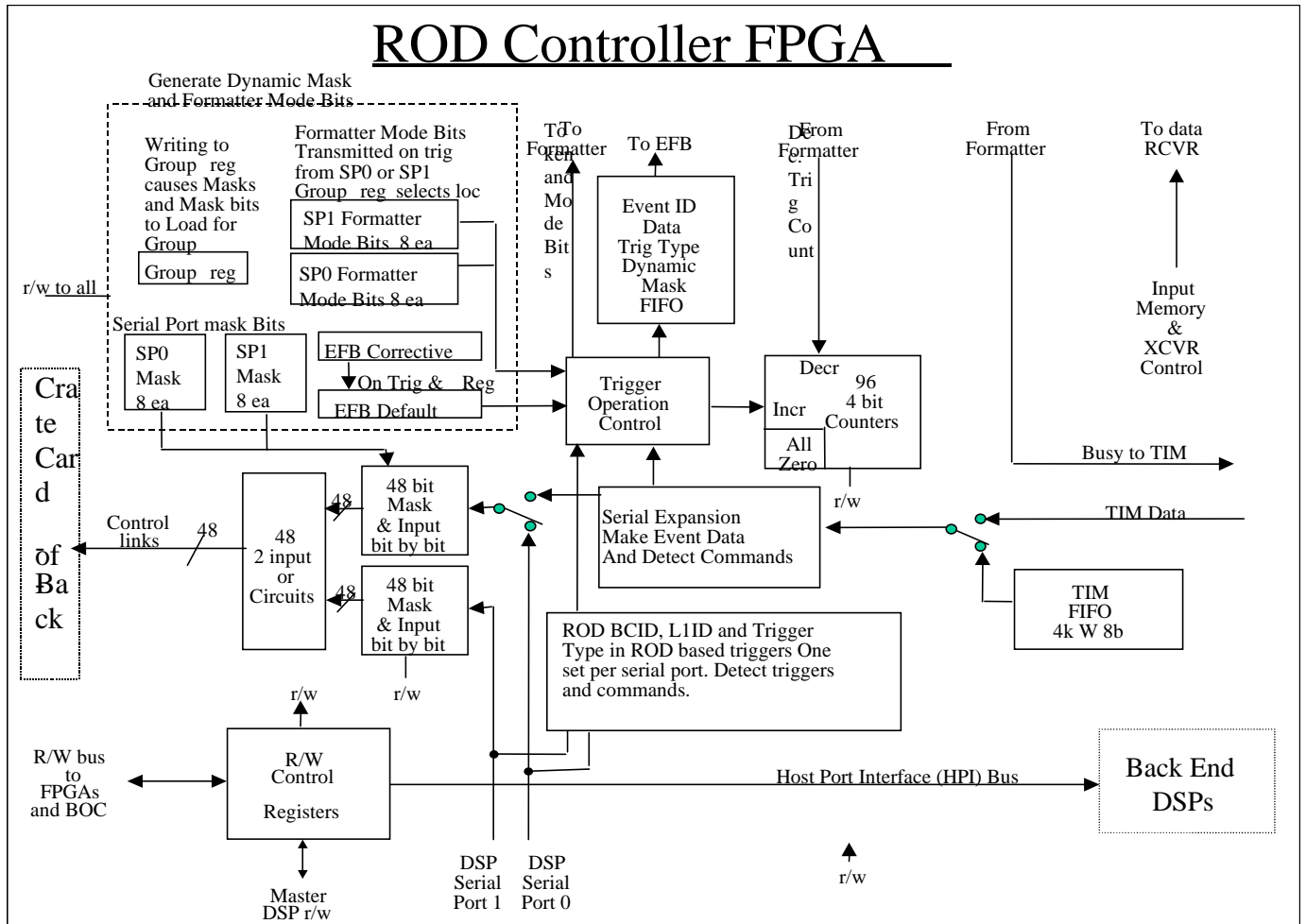
Figure 3: ROD Controller FPGA
